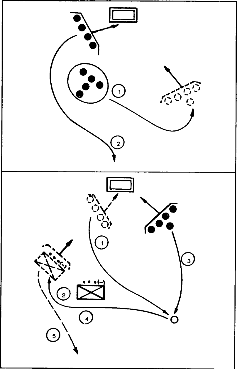
Figure 4-5. Break contact.
